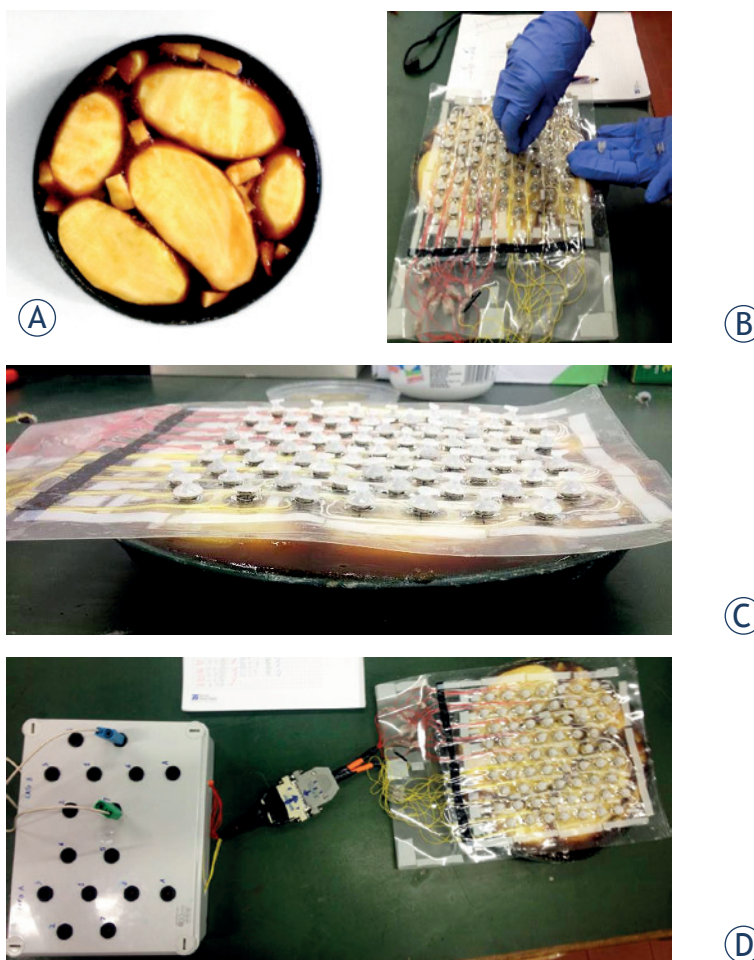
FIGURE 5. (A) Phantom used to test the square flexible electrode with side 15 cm. (B) Manual insertion of needles, (C) device ready for pulse application and (D) connection of the electrode with the connection box.
