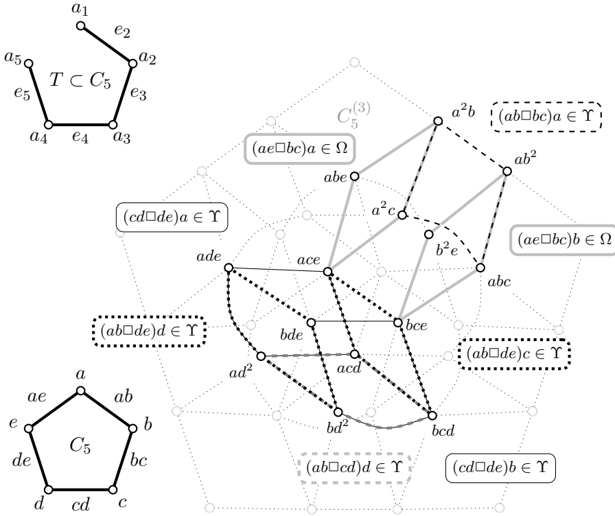
Figure 9: With T as indicated, the sets of squares \Upsilon and \Omega form a basis \mathcal{B} = \Upsilon \cup \Omega of the square space of C_5^{(3)} . Here \Upsilon = \{(ab \square bc)f \mid f \in \{a, b, c\}\} \cup \{(ab \square cd)f, (bc \square cd)f \mid f \in \{a, b, c, d\}\} \cup \{(ab \square de)f, (bc \square de)f, (cd \square de)f \mid f \in \{a, b, c, d, e\}\} . Also \Omega = \{(ae \square ab)f \mid f \in \{a, b\}\} \cup \{(ae \square bc)f \mid f \in \{a, b, c\}\} \cup \{(ae \square cd)f \mid f \in \{a, b, c, d\}\} \cup \{(ae \square de)f \mid f \in \{a, b, c, d, e\}\} . Note |\Upsilon| = 24 and |\Omega| = 14 . The square (ab \square cd)e \notin \mathcal{B} is the “top square” of the Cartesian cube ab \square cd \square de .
