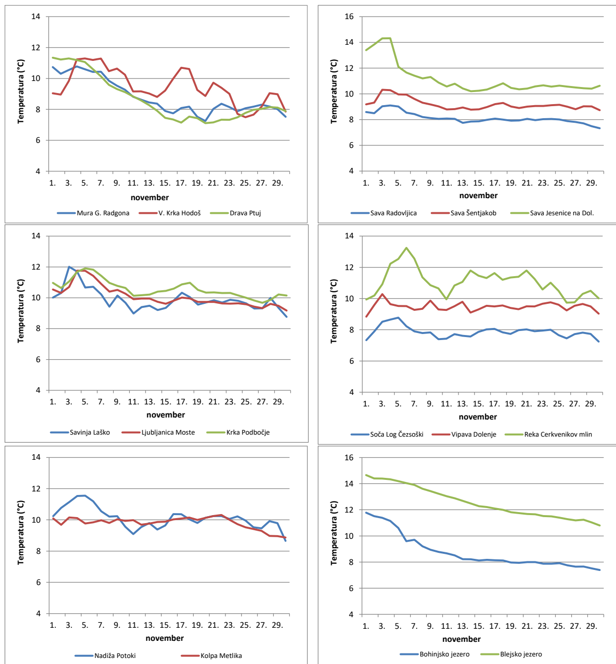
Slika 1. Povprečne dnevne temperature nekaterih slovenskih rek in jezer v novembru 2019, v °C Figure 1. Average daily temperatures of some Slovenian rivers and lakes in November 2019 in °C
