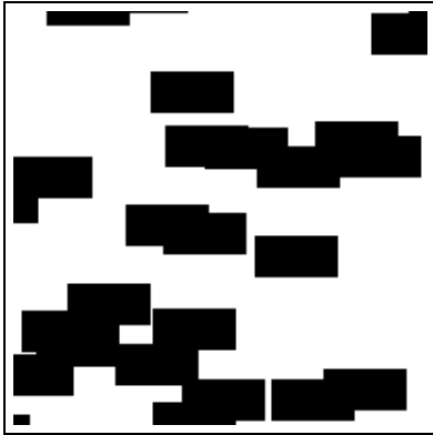
Fig. 4. Realization of \Xi .
