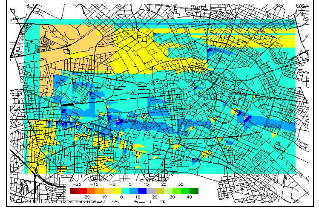
Fig. 19. Residual field \hat{Y}^*(u) .
