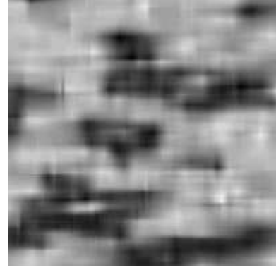
Fig. 12. Residual \hat{Y}^*(u) .
