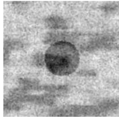
Fig. 13. Extrapolated field \hat{X}(u) .
