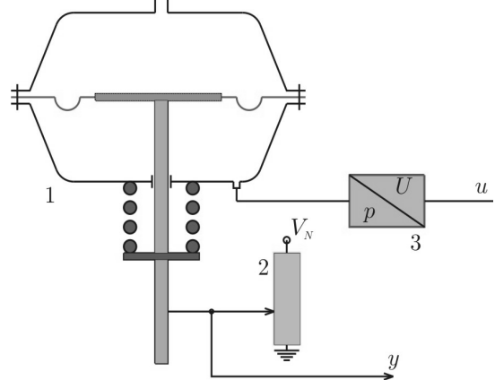
Fig. 2. Electro-pneumatic servo motor
