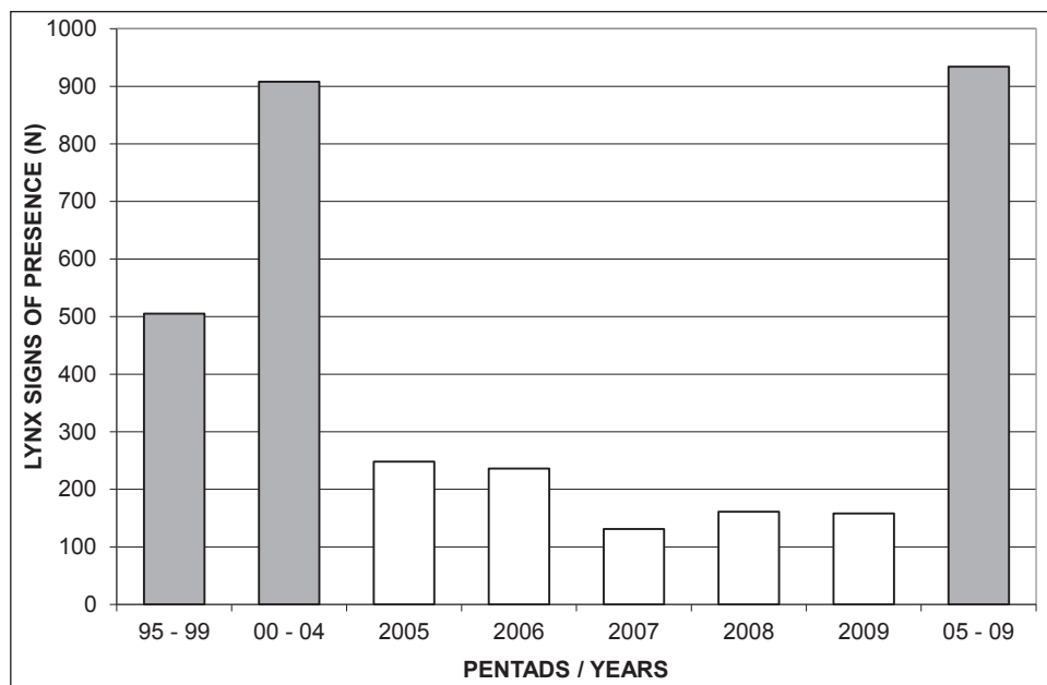
Figure 1: Dynamics of recorded lynx presence data over the pentads between 1995–2009. Lynx presence data in the last pentad – white bars.
