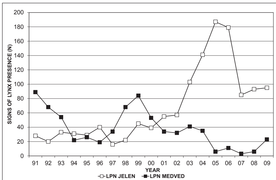
Figure 4: Dynamics of recorded lynx presence data within the monitoring programme in state hunting reserves LPN Jelen and LPN Medved.
