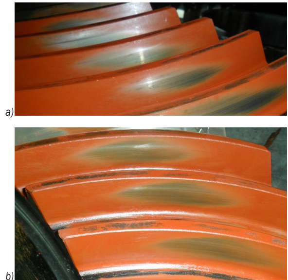
Fig. 10. Tooth bearings on the hypoid gear test machine for the hypoid gear drive 7×43; a) drive side, and b) coast side
