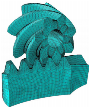
Fig. 8. Finite element model for the hypoid gear drive 7×43
