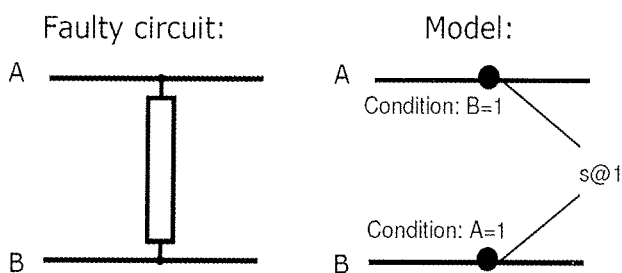
Fig. 2: Example of a conditional stuck-at fault modeling a resistive bridge
