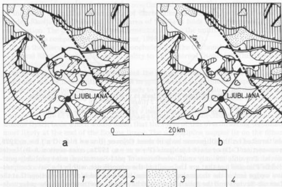
Fig. 8. Course variants of the Southalpine front eastern of the Ljubljana basin 1 Southern Alps; 2 External Dinarides; 3 Tertiary; 4 Ljubljana basin and Ljubljana moor; Explanation of other signs in the legend of fig. 1
