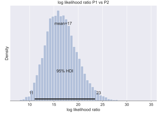
Figure 6: The posterior distribution of log-likelihood ratios for the UNIL dataset along with 95% highest-density intervals to quantify uncertainty.
