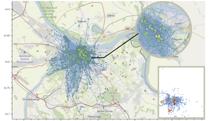
Figure 3: Clustering
