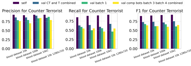
Figure 17: 1280x720 model next to previous models
