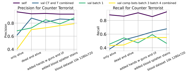
Figure 19: 1280x720 model compared to previous models
