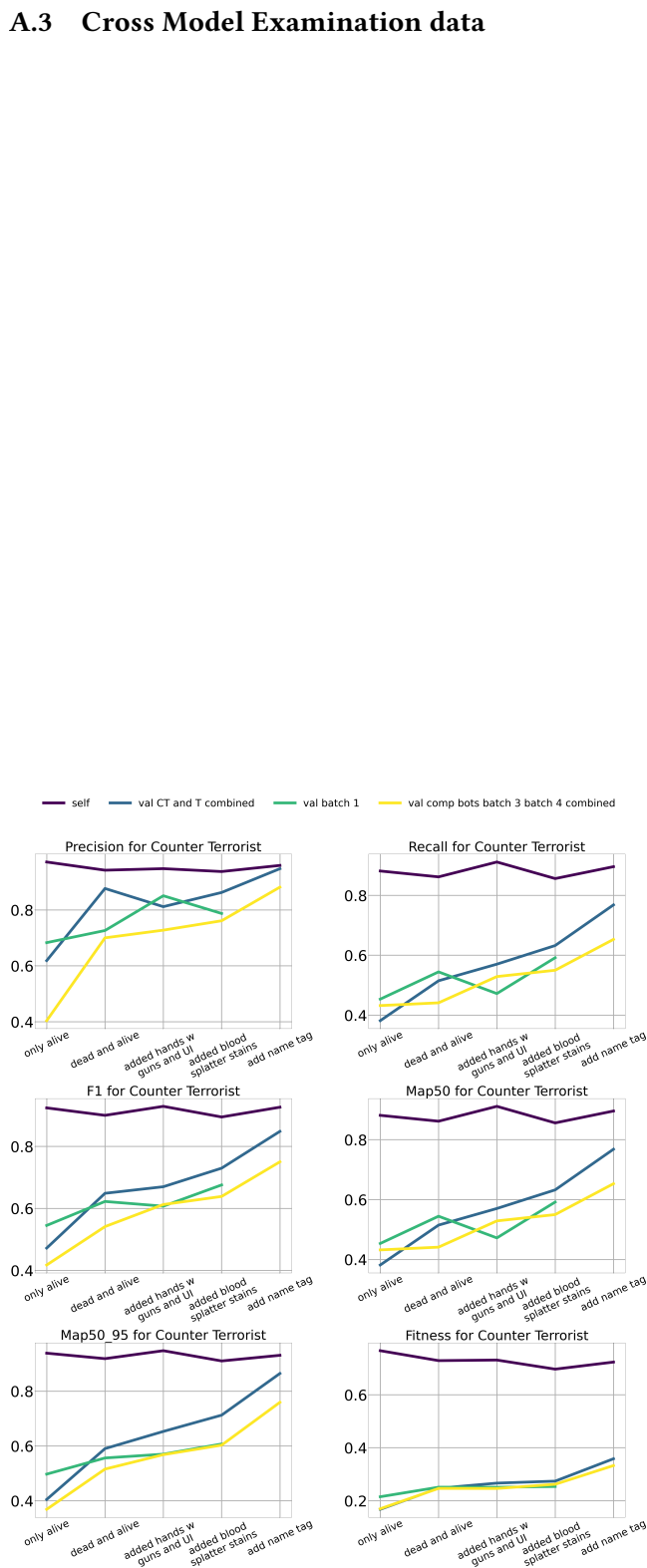
Figure 12: Counter-Terrorist class across all of our generation upgrades
