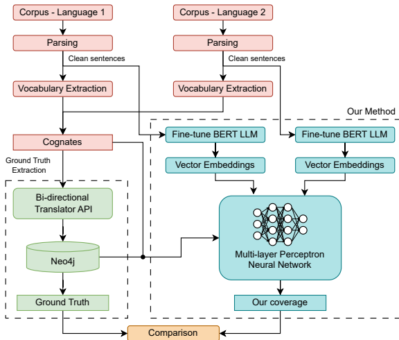
Figure 1: Our methodology
