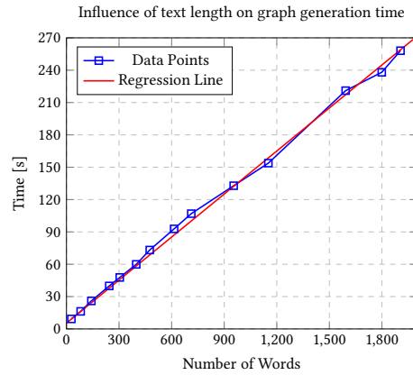
Figure 3: Influence of text length on execution time.
