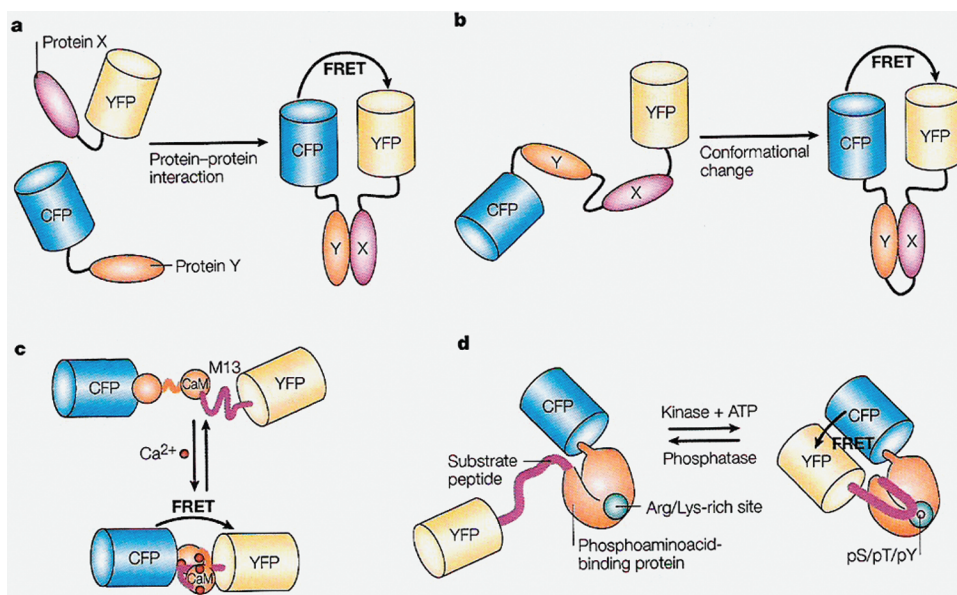
Fig. 3. Application of FRET for monitoring (a) protein-protein interactions, (b) conformational changes within a protein, (c) the presence of \text{Ca}^{2+} and (d) protein phosphorylation. The principles are illustrated using cyan and yellow fluorescent proteins (CFP and YFP) as donors and acceptors, respectively. X and Y denote two different types of proteins (a) and two different domains within the same protein, respectively. In (c) the presence of \text{Ca}^{2+} is detected by means of a fusion protein consisting of a peptide domain M13 recognizing calmodulin bound to \text{Ca}^{2+} . In (d) a substrate peptide is recognized by a specific S, T or Y site of a phosphoaminoacid-binding protein upon its phosphorylation (Arg, arginine; Lys, lysine; pS, phosphoserine; pT, phosphothreonine; pY, phosphotyrosine). Reprinted with permission from Zhang et al (2002).
