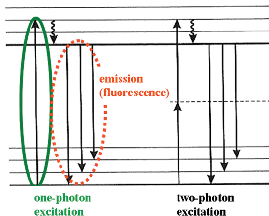
Fig. 2. Molecular energy - level diagram showing one- and two-photon excitation from the ground state to an excited electronic state. For each electronic state there are a number of vibrational levels providing fast relaxation to the lowest vibrational level of the ground- or excited electronic state.
