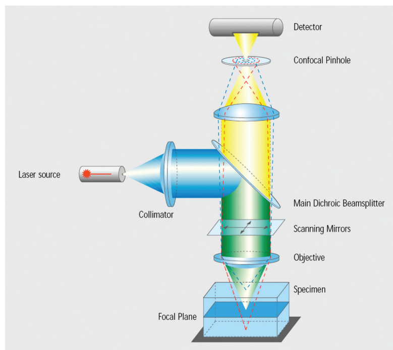
Fig. 1. The principle of a confocal microscopy setup. Light from a laser point source is reflected off a dichroic mirror and imaged onto the specimen. Only fluorescence light emitted from the focal plane is detected since out-of-focus light is unable to pass through the pinhole. Reproduced with permission from Simbürger et al (2006).
