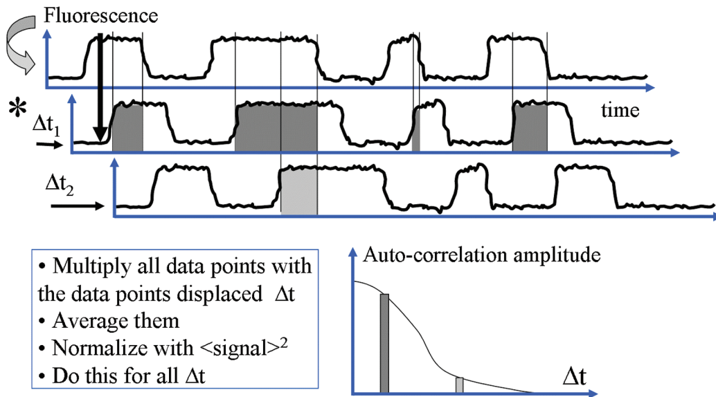
Fig. 5. Steps involved in the construction of an FCS auto-correlation curve; the fluorescence time trace is displaced by an amount \Delta t and data points from the two traces are pairwise multiplied to create a new trace which is averaged over all time points and normalized wrt. the squared average of the original signal ( \langle \text{signal} \rangle^2 ; averaged over all time points). Shown are two examples with \Delta t = \Delta t_1 and \Delta t = \Delta t_2 . Reproduced with permission from R. Schmauder.
