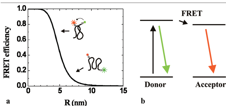
Fig. 4. (a) FRET efficiency as a function of donor-acceptor distance for a FRET pair with R_0 = 5 nm and (b) sketch of the electronic energy level diagram of donor and acceptor; the transfer of excitation energy is indicated with a black arrow, and the donor and acceptor fluorescence emissions with green and red arrows, respectively.
