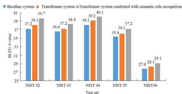
Figure 1: Comparison of bLEU-4 values.
