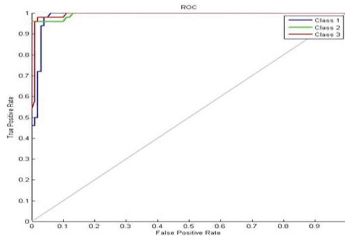
Fig. 8. ROC for detecting benign and malignant tumor using PNN classifier.
