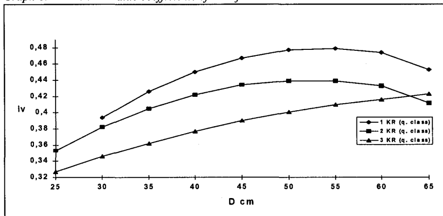
Graph 6: Fitted value coefficients of data from Bosnia
