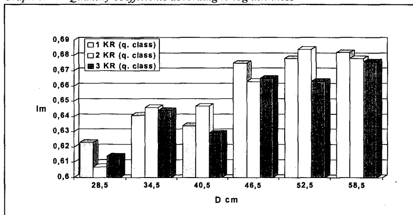
Graph 1: Quantity coefficients according to log thickness
