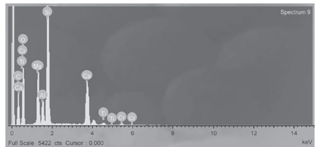
Fig. 14. X-ray spectrum of presumed Al-rich diopside (Sp. 9 - spectrum 9)
