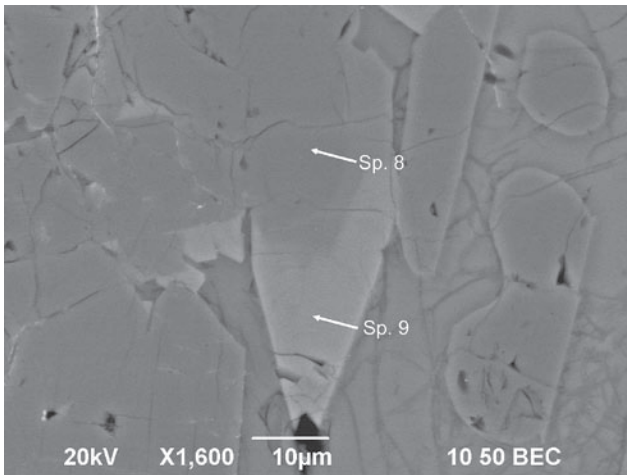
Fig. 12. BSE image of olivine (forsterite) (Sp. 8 - spectrum 8) and presumably Al-rich diopside (Sp. 9 - spectrum 9) in a BO chondrule
