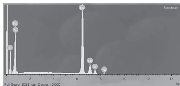
Fig. 3. X-ray spectrum of kamacite (Sp. 1 - spectrum 1) Sl. 3. Spekter kamacita (Sp. 1 - spectrum 1)
