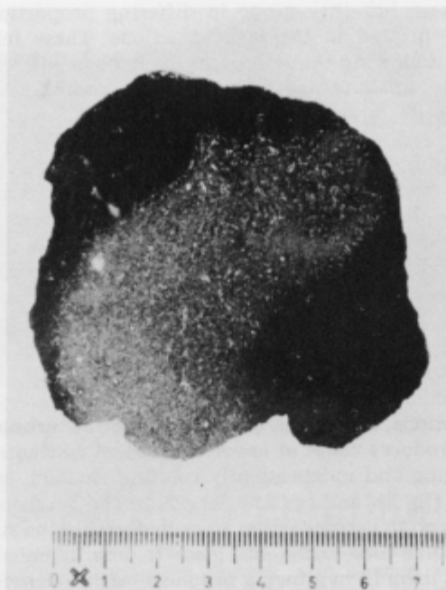
Fig. 1. Hand-specimen showing a whirling felsic portion in the surrounding basaltic magma. Scale in cm
