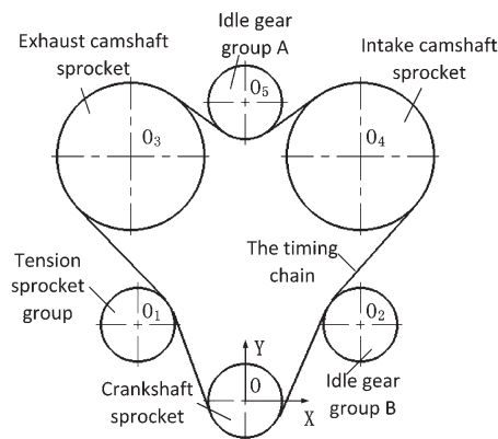
Fig. 1. The structure of timing silent chain system
