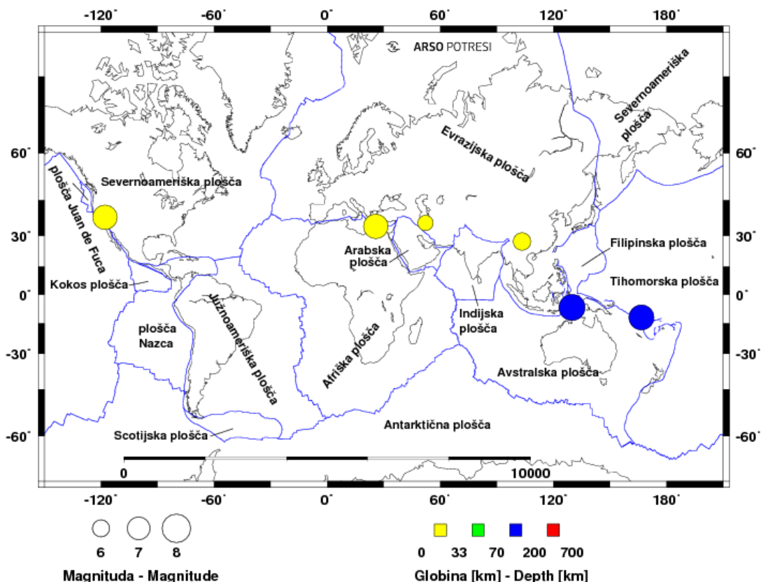
Figure 1. The world strongest earthquakes, May 2020
