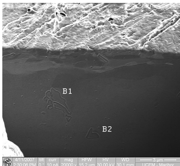
Figure 2: An overview of the Al surface and the direct area under the surface before irradiation with the laser beam. A thin and partly recrystallized surface layer is visible.
