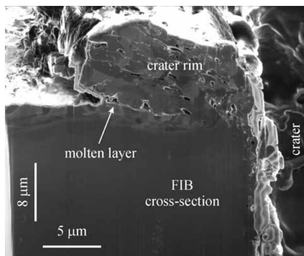
Figure 7: The Rayleigh-Taylor instability is visible on the side of the "deep" crater
