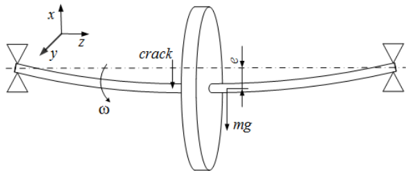
Fig. 1. Jeffcott rotor model with a lateral crack
