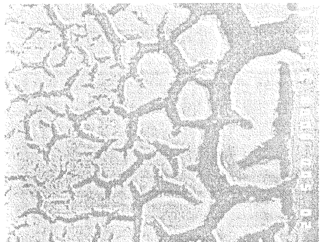
Figure 5: Metallization perforated by cracks (paste containing 2,5 at% Ti, firing temperature: 850 °C, dwell time: 30 minutes, firing atmosphere: argon, film thickness: 25-30 \mu\text{m} ).
