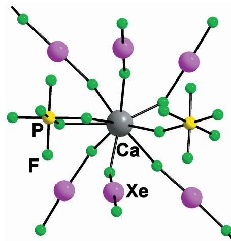
Figure 9. Example of the metal coordinated by non-bridging and bridging molecules of \text{XeF}_2 ; [\text{Ca}(\text{XeF}_2)_5](\text{PF}_6)_2 72
