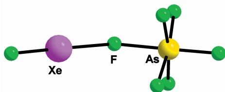
Figure 4. Structure of \text{XeFAsF}_6 57
