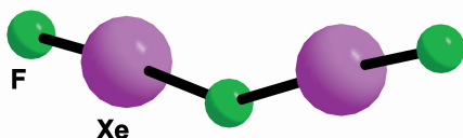
Figure 3. V-shaped cation \text{Xe}_2\text{F}_3^+ in the compounds \text{Xe}_2\text{F}_3\text{AF}_6 (A = As, Sb, Ru)
