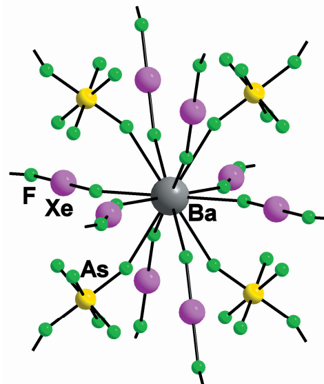
Figure 10. Example of the metal coordinated by bridging molecules of \text{XeF}_2 ; [\text{Ba}(\text{XeF}_2)_5](\text{AsF}_6)_2
