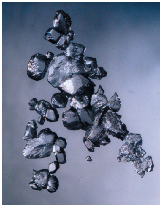
Figure 2. Crystals of \text{XeF}_2
