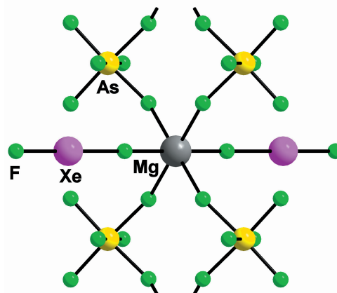
Figure 7. Example of the metal coordinated by non-bridging molecules of \text{XeF}_2 ; [\text{Mg}(\text{XeF}_2)_2](\text{AsF}_6)_2 73
