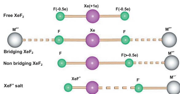
Figure 6. \text{XeF}_2 on the ionization pathway from “free” molecule to the \text{XeF}^+ cation
