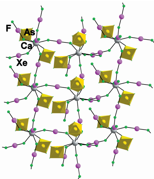
Figure 8. Layer structure in the [\text{Ca}(\text{XeF}_2)_4](\text{AsF}_6)_2 71
