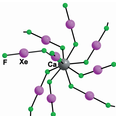
Figure 11. Example of the metal coordinated only by \text{XeF}_2 (bridging and non-bridging); one \text{Ca}^{2+} centre in [\text{Ca}_2(\text{XeF}_2)_9](\text{AsF}_6^-)_4 . 74
