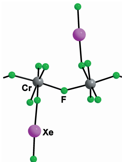
Figure 5. Structure of the \text{XeF}_2\cdot\text{CrF}_4 63
