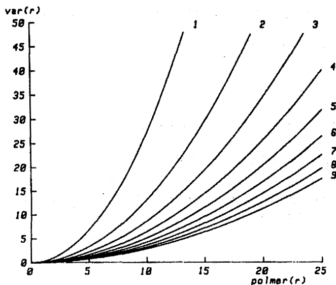
Slika 3: Variance zaporednih razmikov ( \sigma^2_{r_k} ) glede na velikost razmika r_k Figure 3: The ratio between r_k and \sigma^2_r in the Poisson forest
