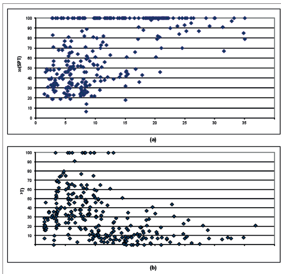
Fig. 5: List of SPT values with the depth: (a) Non-karstified land. (b) Karstified land
