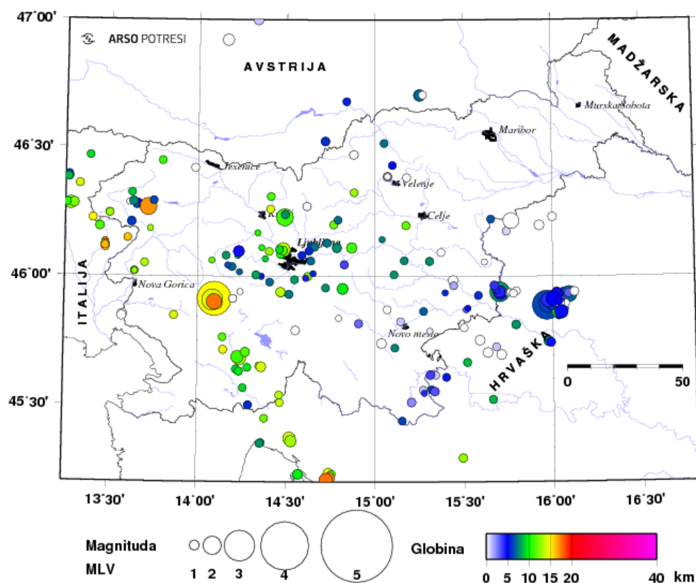
Slika 1. Potresi v Sloveniji, april 2020 Figure 1. Earthquakes in Slovenia, April 2020
