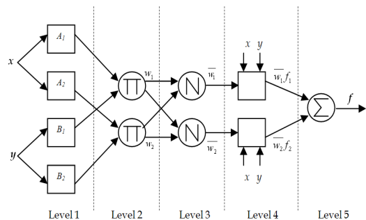
Fig. 7. Characteristic structure of the neuro-fuzzy system
