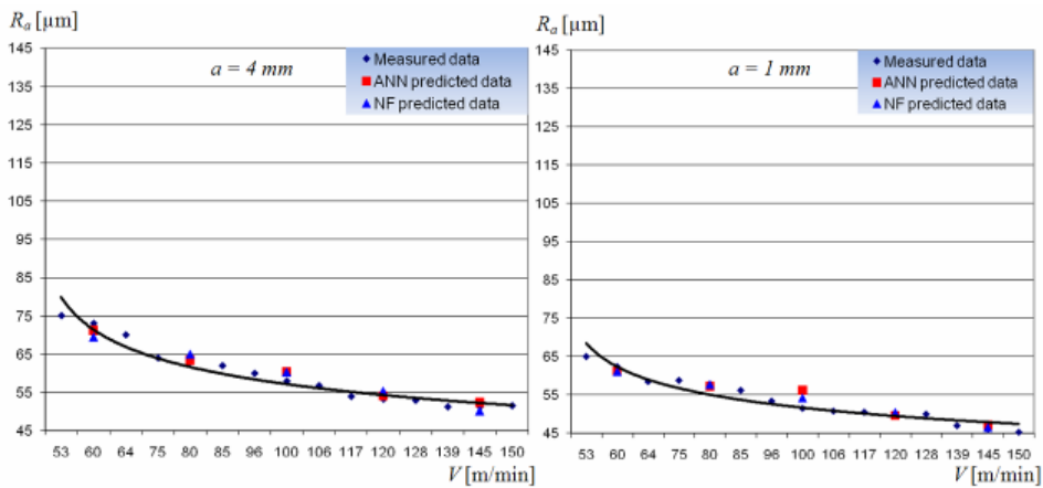
Fig. 11. Measured, ANN and NF predicted values of the arithmetic mean deviation ( f = 0.135 mm/rev)
