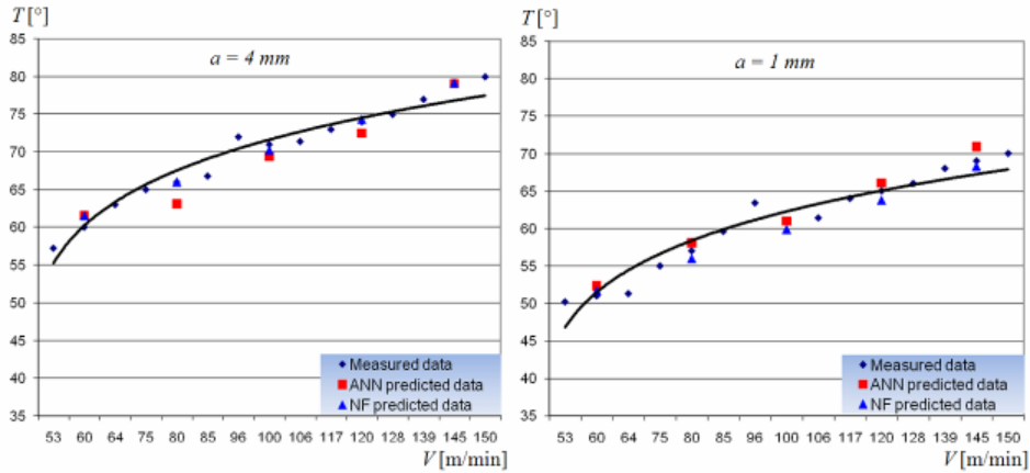
Fig. 9. Measured, ANN and NF predicted values of the workpiece temperature ( f = 0.135 mm/rev)
