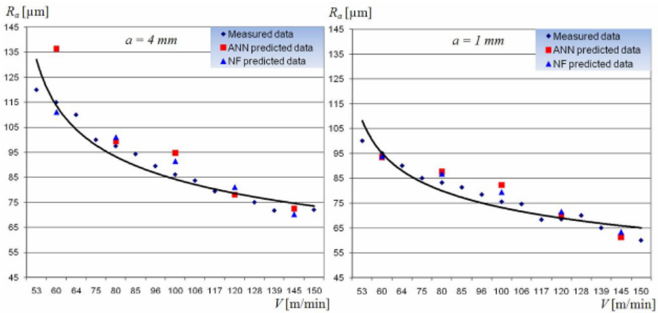
Fig. 10. Measured, ANN and NF predicted values of the arithmetic mean deviation ( f = 0.224 mm/rev)
