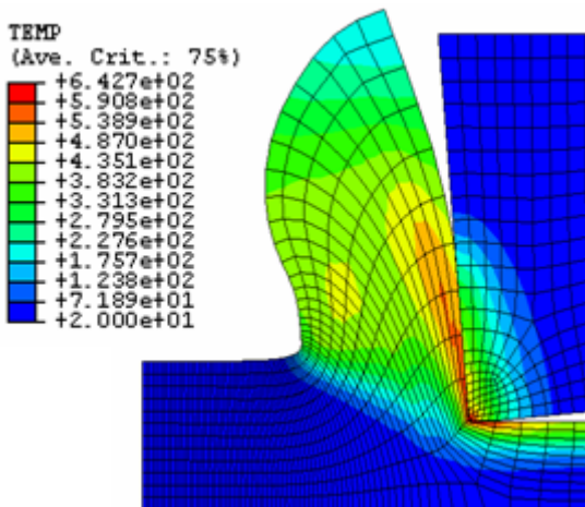
Fig. 3. Temperature contours by arbitrary Lagrangian eulerian method
