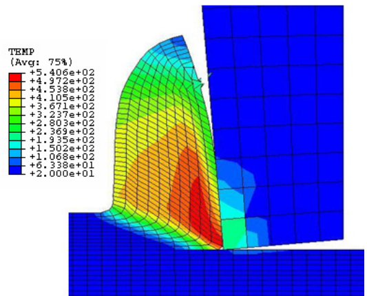
Fig. 5. Temperature contours by node debond method
