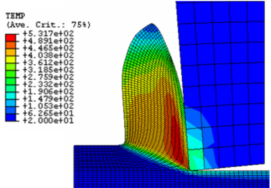
Fig. 4. Temperature contours by element deletion method
