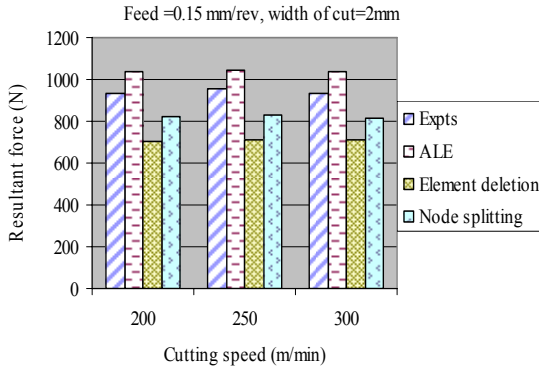
Fig. 1. Resultant forces obtained in turning operations by experiments and simulations, feed = 0.15 mm/rev, width of cut = 2mm
