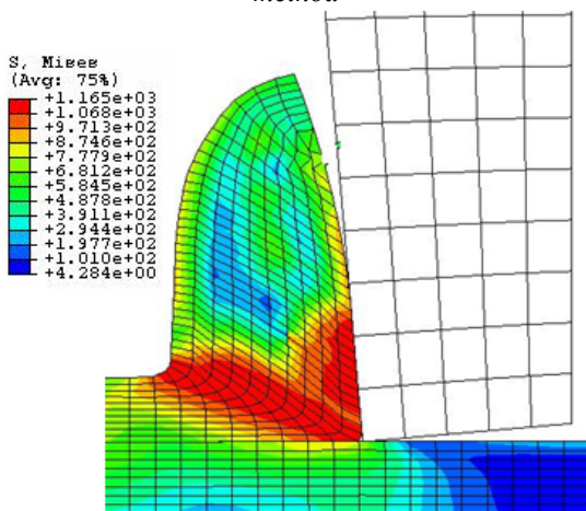
Fig. 7. Mises stress contours by element deletion method
