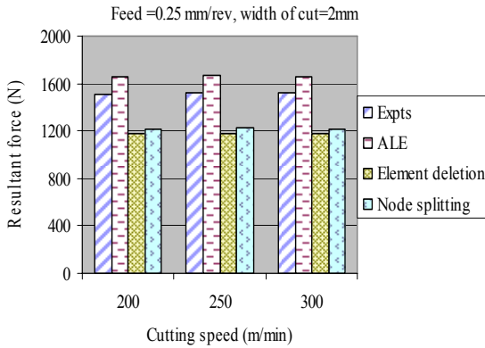
Fig. 2. Resultant forces obtained in turning operations by experiments and simulations, feed = 0.25 mm/rev, width of cut = 2mm
