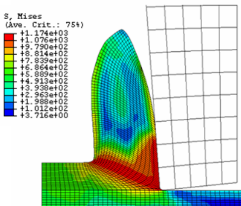
Fig. 7. Mises stress contours by element deletion method
