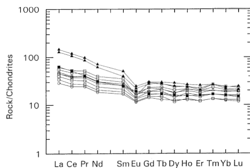
Fig. 3. Chondrite normalised REE abundance for the samples from Trlično (closed triangles) and andesite from Zagaj at Rogaska Slatina (closed square) and the Smrekovec volcanic rocks (open squares, triangles, circles)
