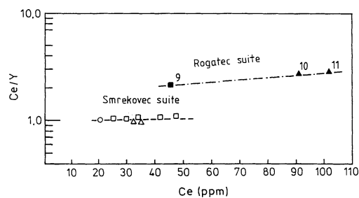
Fig. 4. The Ce/Y vs. Ce diagram with the samples from Trlično (10, 11) and Zagaj at Rogaska Slatina (9) and the Smrekovec volcanic rocks (open squares, triangles and a circle)
