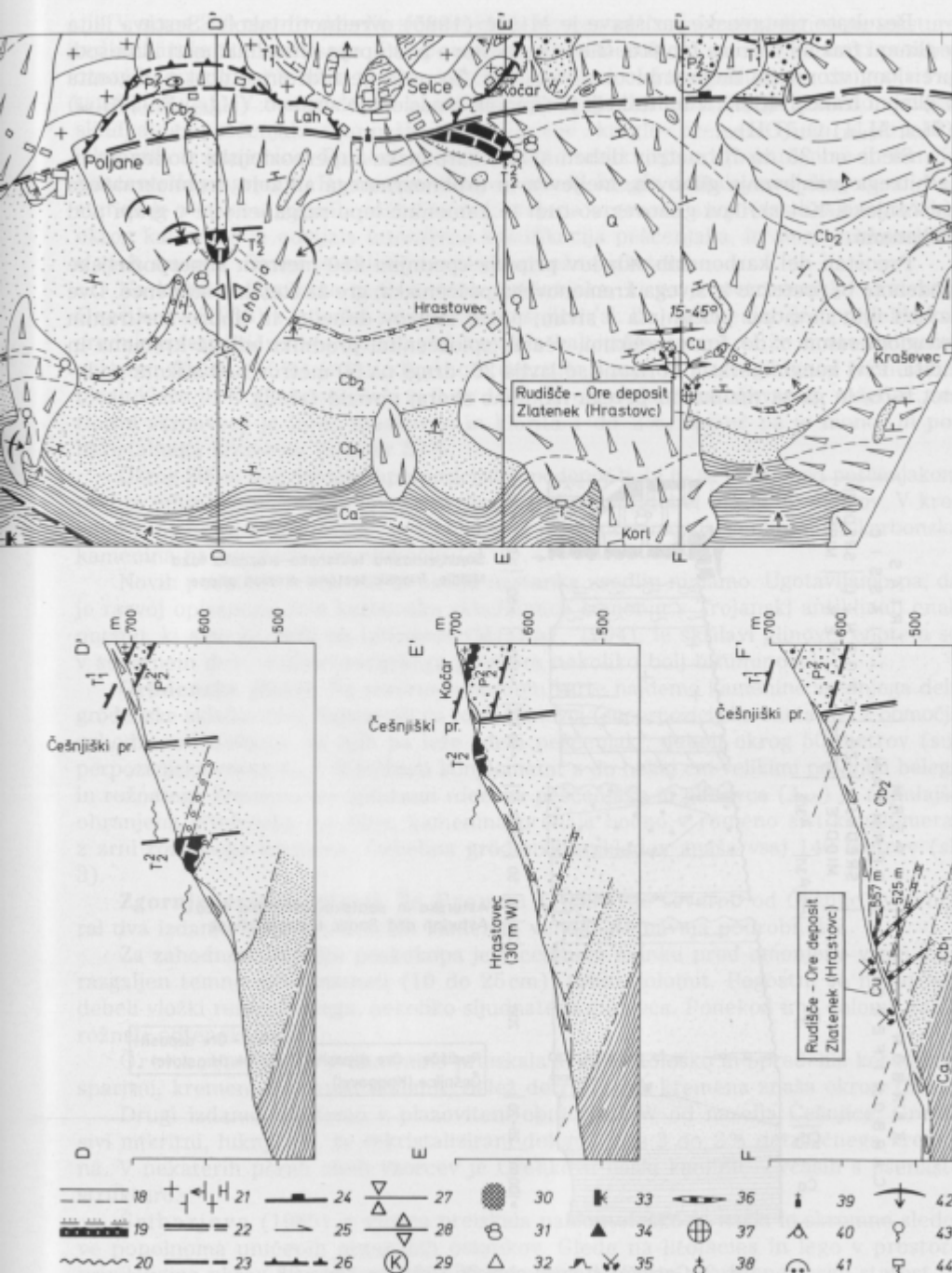
Fig. 2. Geological map of the Češnjice-Zlatenec areas (a) and geological cross sections (b)
