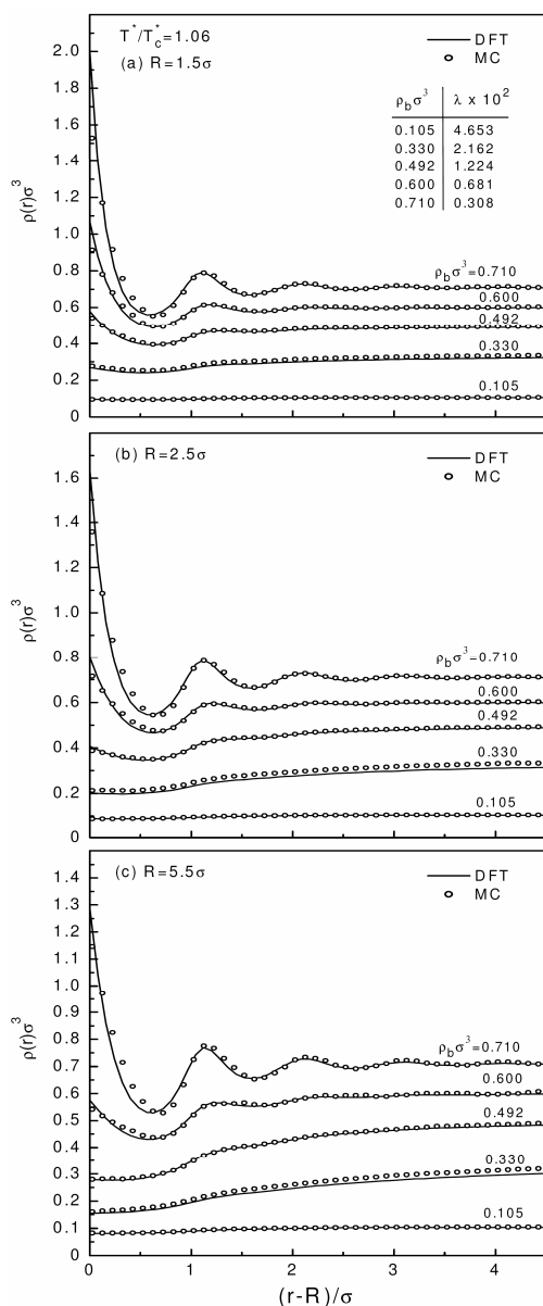
Figure 1. Monte Carlo (symbols) and density functional (lines) results for the density profiles of the LJ fluid near a large spherical particle of effective radius R = 1.5\sigma (a), R = 2.5\sigma (b), and R = 5.5\sigma (c), at the supercritical reduced temperature T^*/T_c^* = 1.06 and at different values of the bulk reduced density. \lambda is the adjustable parameter determined by the single hard wall sum rule considering the contact theorem using the exact simulation results for the contact densities.
