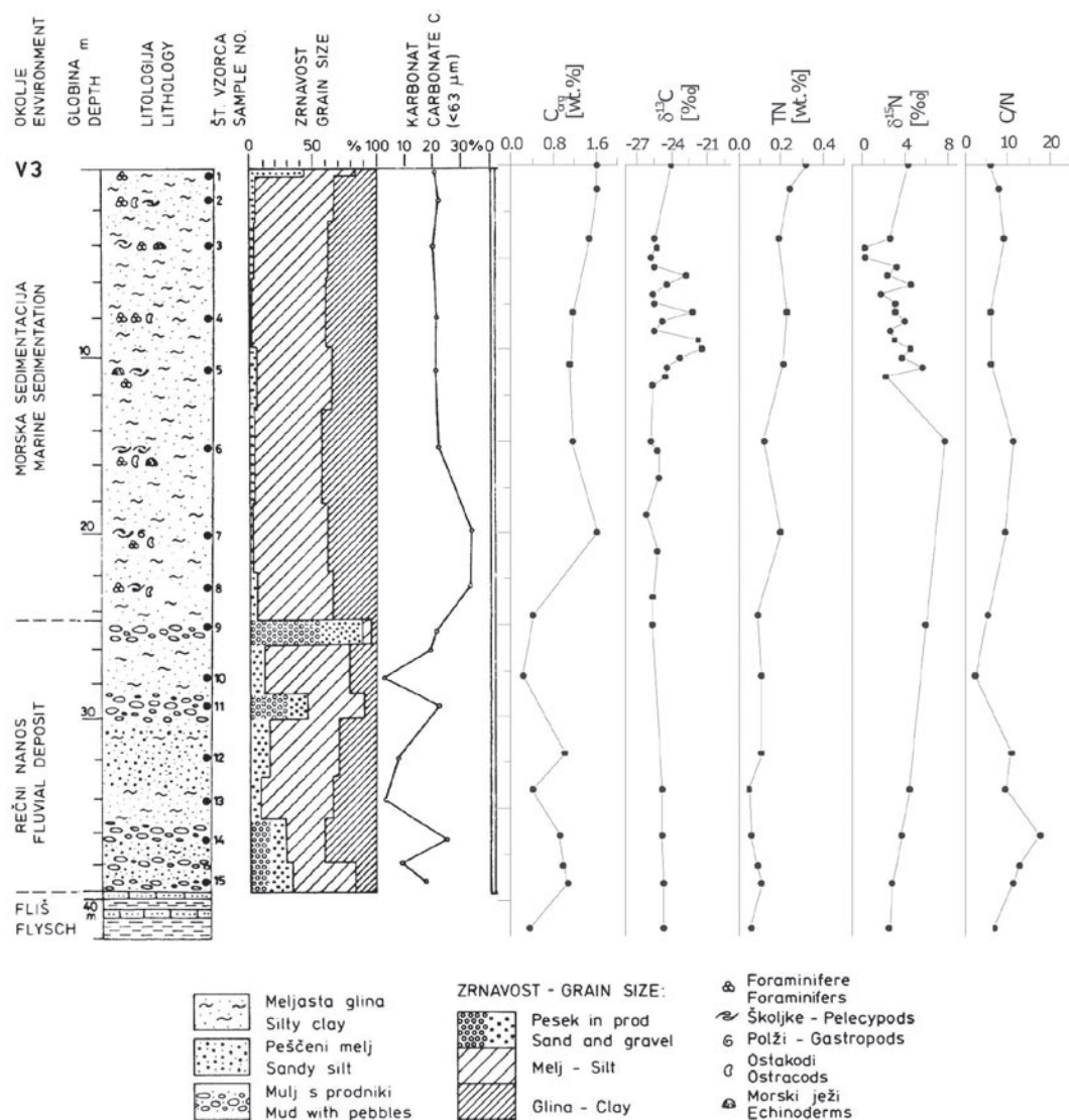
Figure 3. Vertical profiles of lithology, grain size, carbonate content, (Ogorelec et al., 1984, 1987), organic carbon ( C_{org} ) (Faganeli et al. 1987), \delta^{13}C_{org} , total nitrogen (TN), \delta^{15}N values and C/N ratios in the sediment core V-3.
