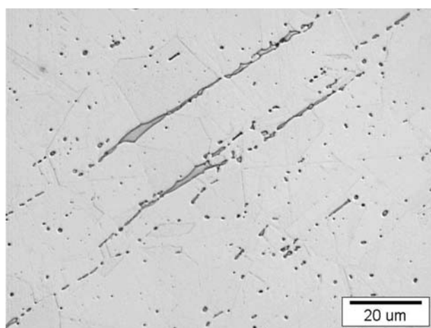
Figure 6: Microstructure of austenitic stainless steel AISI 304 with elongated delta ferrite. In deformed regions the deformation-induced martensite was also present. Etched with aqua regia.
