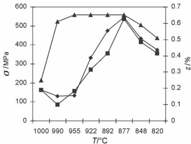
Figure 8: Evolution of internal stresses (weld ◆, base material ■) and coefficient of plastic extension Z (▲) with respect to the processing temperature.
