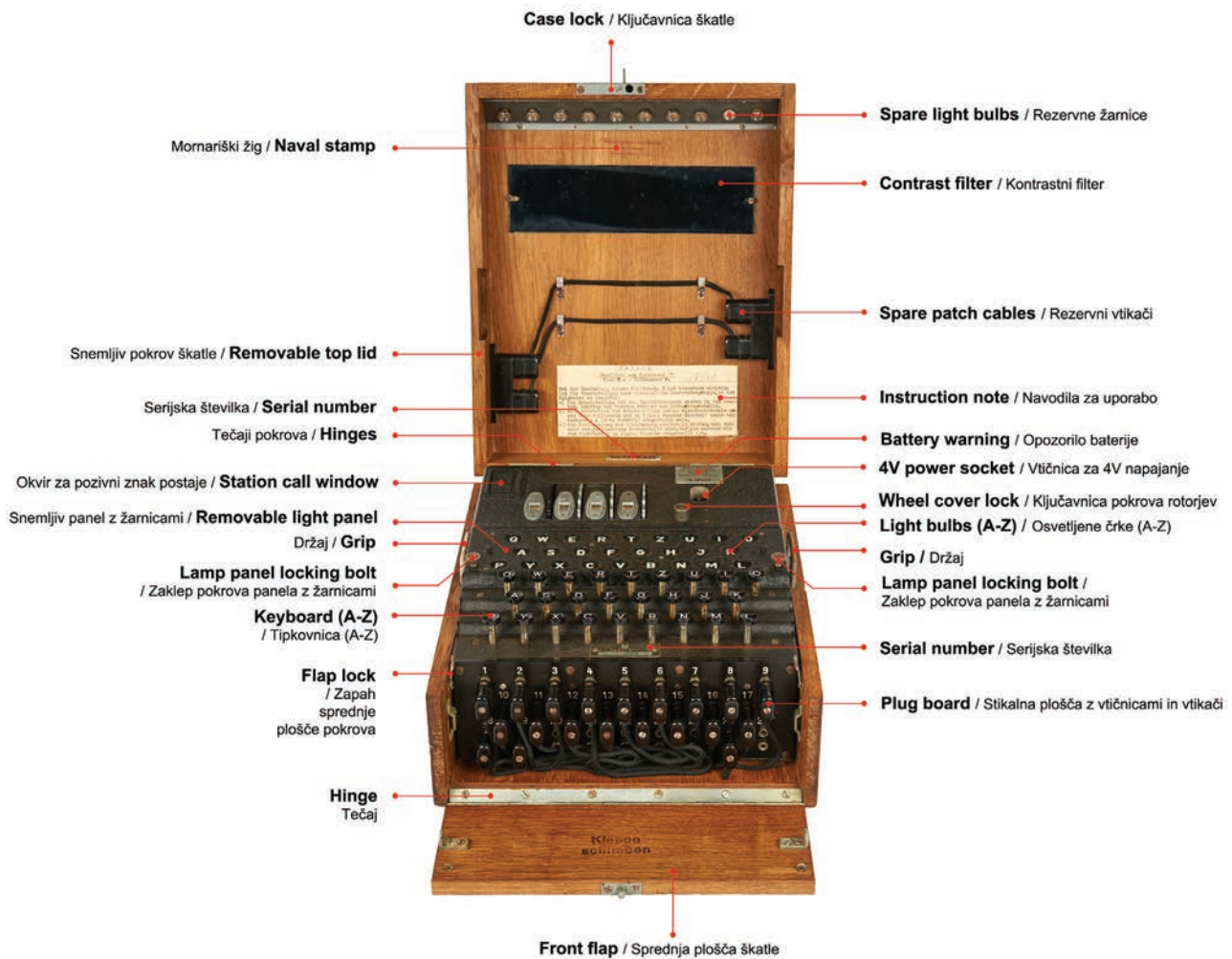
Figure 13: Enigma M4. Machine parts (Source: Cryptomuseum, 2022).
