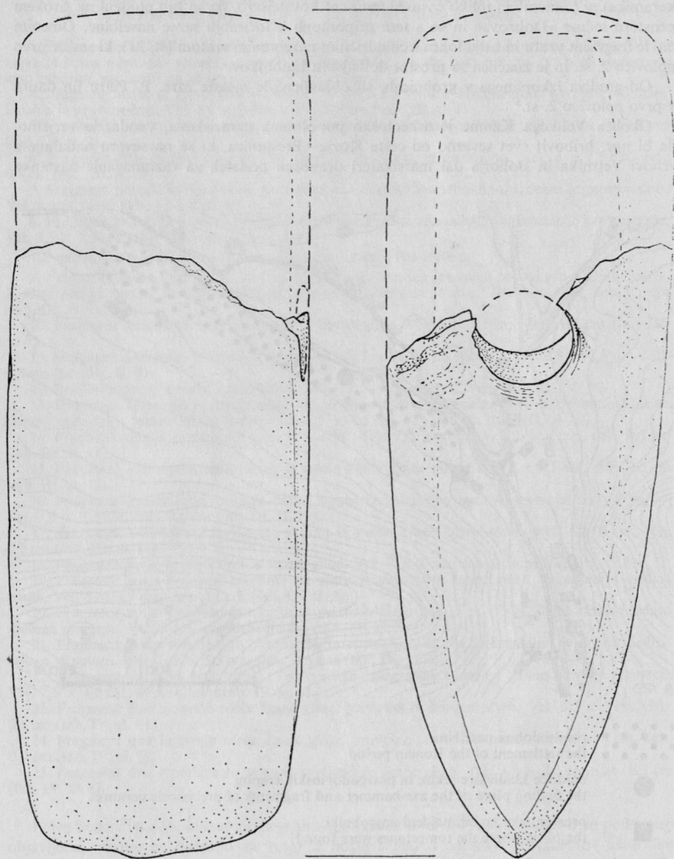
Sl. 6. Veliki Kamen, kladivasta sekira (risala D. Lunder). Merilo 1 : 1 Fig. 6. Veliki Kamen, axe-hammer (designed by D. Lunder). Scale 1 : 1
