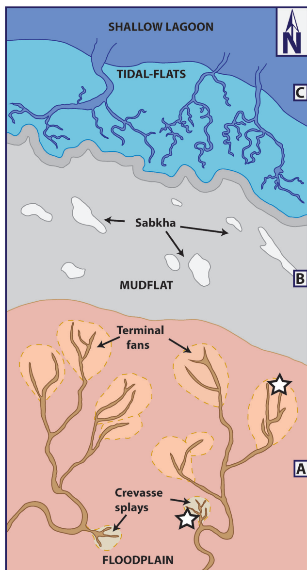
Fig. 7. Schematic paleoenvironmental reconstruction of the Travenanzes Formation (modified from BREDÁ & PRETO, 2011) A = aluvial plain with river channels, terminal fans, crevasse splays and a flood plain; B = Mudflat and coastal sabkha; C = Carbonate tidal flats and shallow lagoons. The stars mark the two most likely locations of the Lesno Brdo area.
