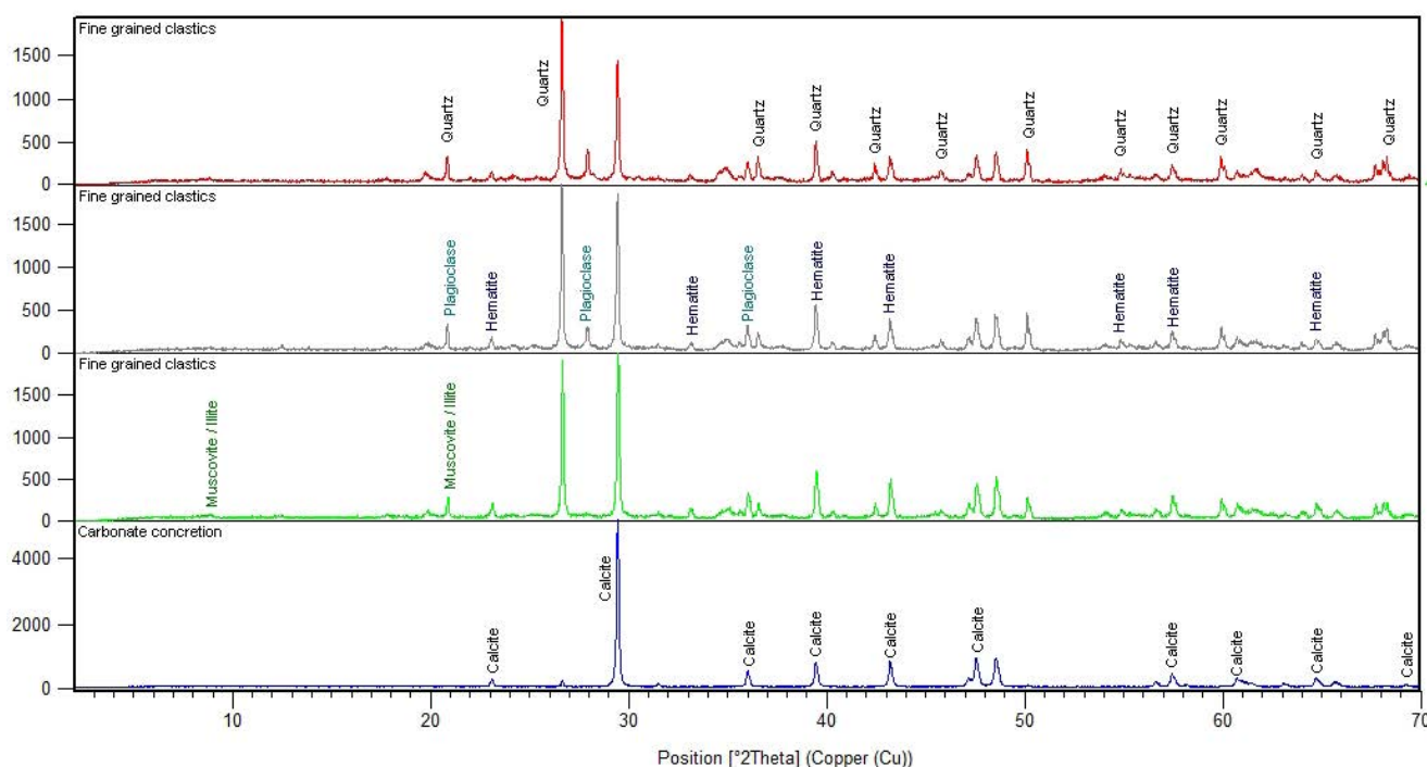
Fig. 6. Diffractograms of fine-grained clastites (upper three) and carbonate concretion (below).
