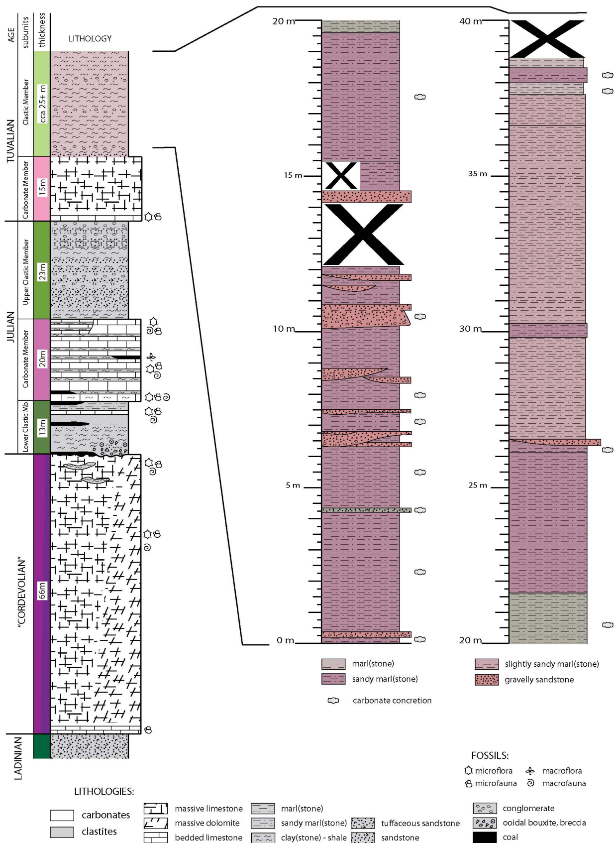
Fig. 3. Carnian succession of the Dinaric Carbonate Platform at Lesno Brdo (modified from: JELEN, 1990) with an investigated section of the Tuvalian clastic member.
