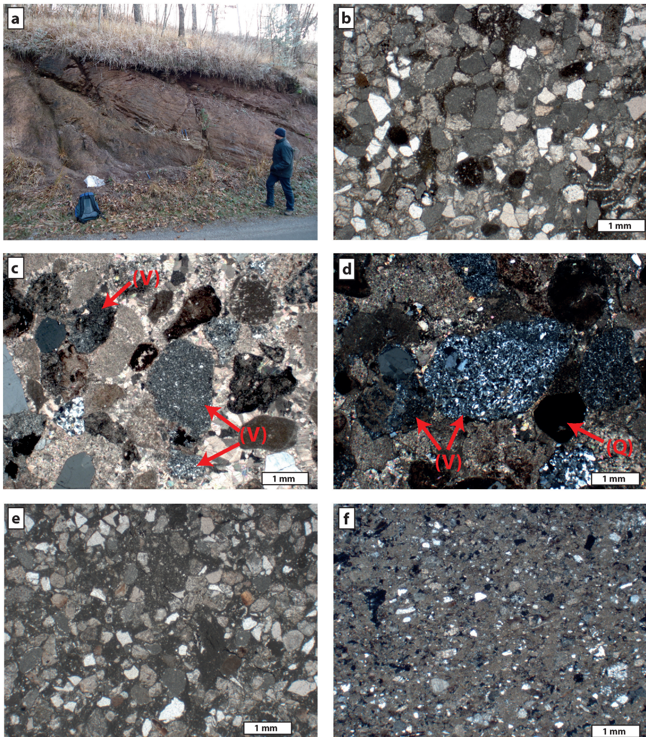
Fig. 4. Facies of the Tuvlian clastic member at Lesno Brdo. a) Lower part of the section in which sandy marlstone is interbedded with channels of gravelly sandstone. b) Medium- grained sandstone with quartz grains and carbonate lithoclasts. c) medium- to coarse-grained sandstone with various carbonate lithoclasts, quartz grains and lithoclasts of vulcanics (V); some carbonate grains contain opaque mineral (cross-polarized light). d) Pebbly sandstone with lithoclasts of vulcanics (V) with microcrystalline matrix and quartz and feldspar phenocrysts; various carbonate lithoclasts are also present; in the lower-right corner of the micrograph a monocrystal quartz grain is marked (Q) (cross-polarized light). e) Fine- to medium-grained sandstone composed predominantly of carbonate lithoclasts and monocrystal quartz grains; at margins of particular carbonate grains thin monocrystal quartz occurs. f) Sandy siltstone in which some grains up to 0.2 mm are visible – mostly quartz, carbonate lithoclasts and some lithoclasts of vulcanics (cross-polarized light).
