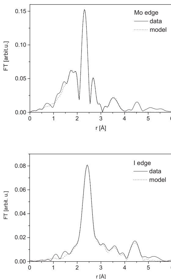
Figure 5. Comprehensive EXAFS model of \text{Mo}_6\text{S}_3\text{I}_6 for the Mo and I edge.
