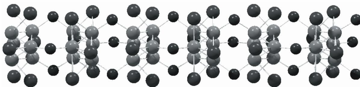
Figure 4. The proposed structure: six Mo octahedra (grey) of the polymer chain are shown, dressed and coupled with S (black-small) and I ions (black-large). The partition of the anions between the two sites may vary with stoichiometry.
