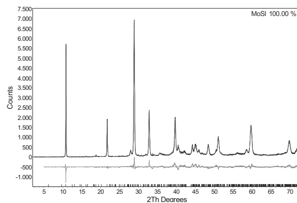
Figure 1. The XRD scan of the \text{Mo}_6\text{S}_3\text{I}_6 nanowire sample (x-axis – Bragg angle 2\theta ). The residue of the Rietveld fit is shown below (for details see reference 2).
