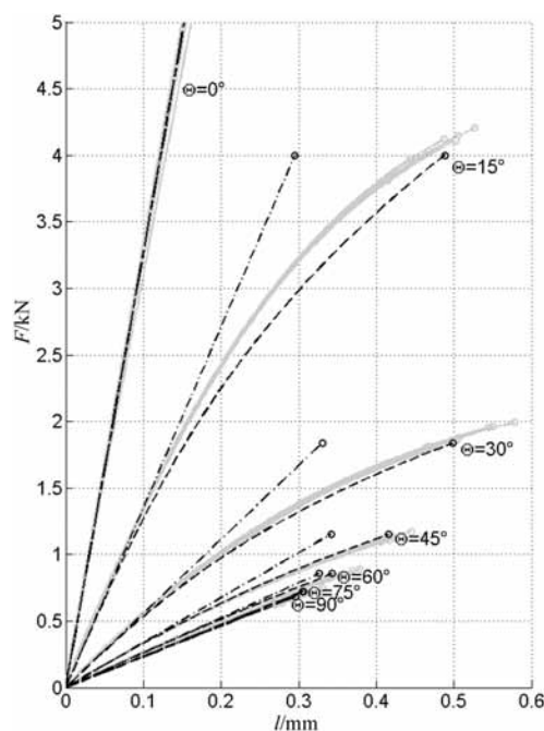
Figure 3: Force-displacement diagram (gray – experiment, dashed – FEM non-linear, dash-and-dot – FEM linear)
