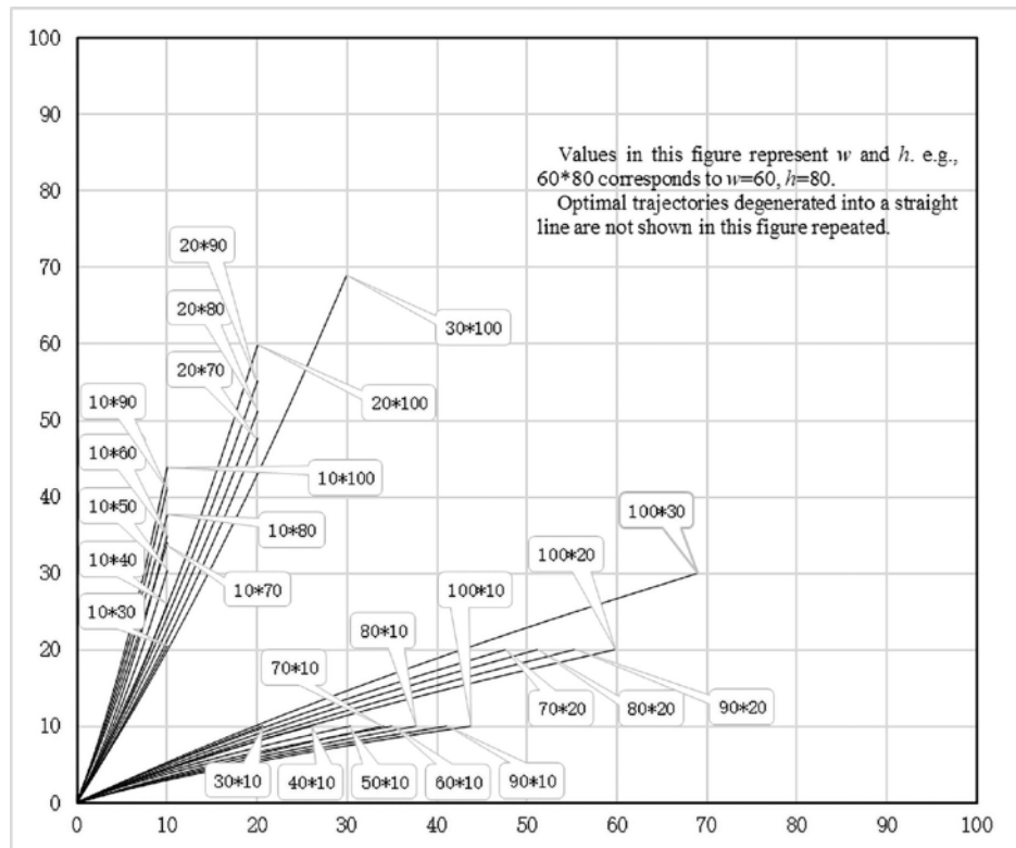
Fig. 10 Optimal main aisle trajectory map of parabolic Fishbone of 100 warehouses
