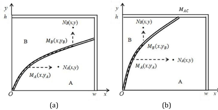
Fig. 5 Two sub-forms of parabolic Fishbone layout
