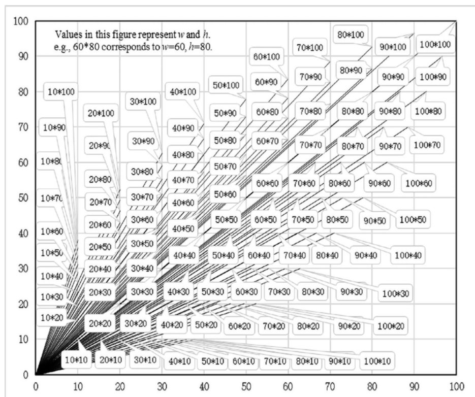
Fig. 11 Optimal main aisle trajectory map of straight Fishbone of 100 warehouses
