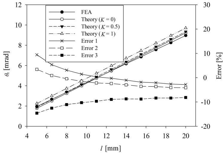
Fig. 3. Variation of \theta_x according to length l under torsion T_x
