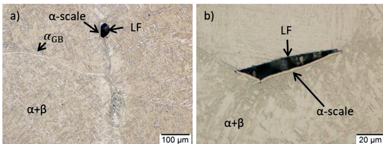
Figure 4: LM image of remaining \alpha -scale in lack-of-fusion pore on the DED side of HAM x a) and HAM z b) parts (LF-Lack of Fusion pores)
