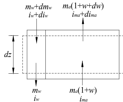
Fig. 2. Control volume of SCT
