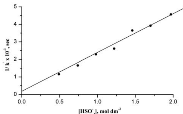
Figure 3: Plot of 1/k' as a function of concentration of \text{HSO}_4^- ions.
