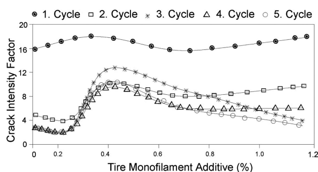
Figure 7: CIF for Avanos clay amended with tire monofilaments
