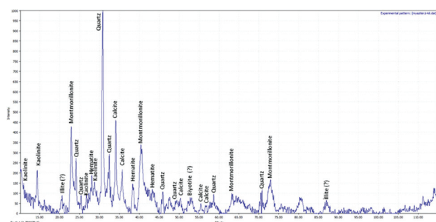
Figure 1: The mineralogical composition of the Avanos Clay
