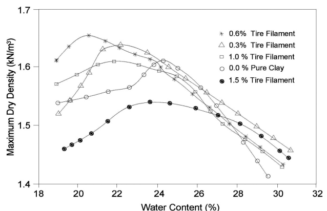
Figure 5: Compaction characteristics of mixed Avanos clay
