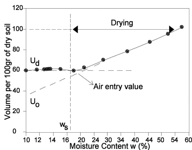
Figure 2: Shrinkage curve for Avanos solo clay
