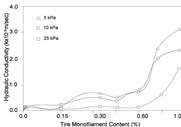
Figure 6: Hydraulic conductivity of mixed Avanos clay
