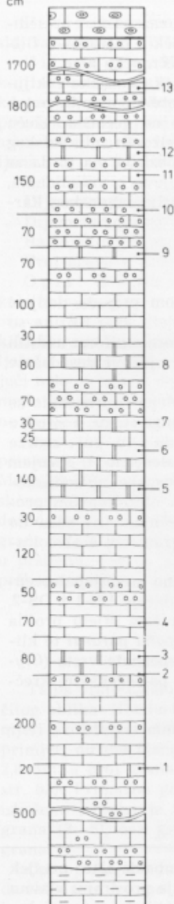
Sl. 1. Geološki stub u miliolidskim krečnjacima i geološka karta okoline Slivja Fig. 1. Geological column in miliolid limestones and geological map of environs of Slivje
