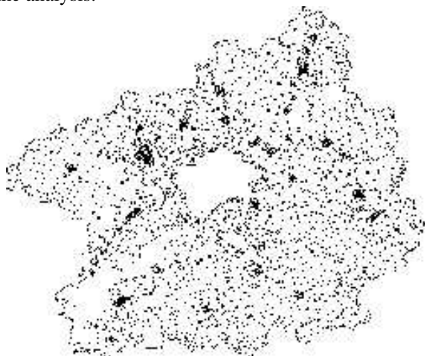
Fig. 3. Population at 3582 administrative units in Central Bohemia represented by discs (see the text in the subsection Description of data and problem setting).
