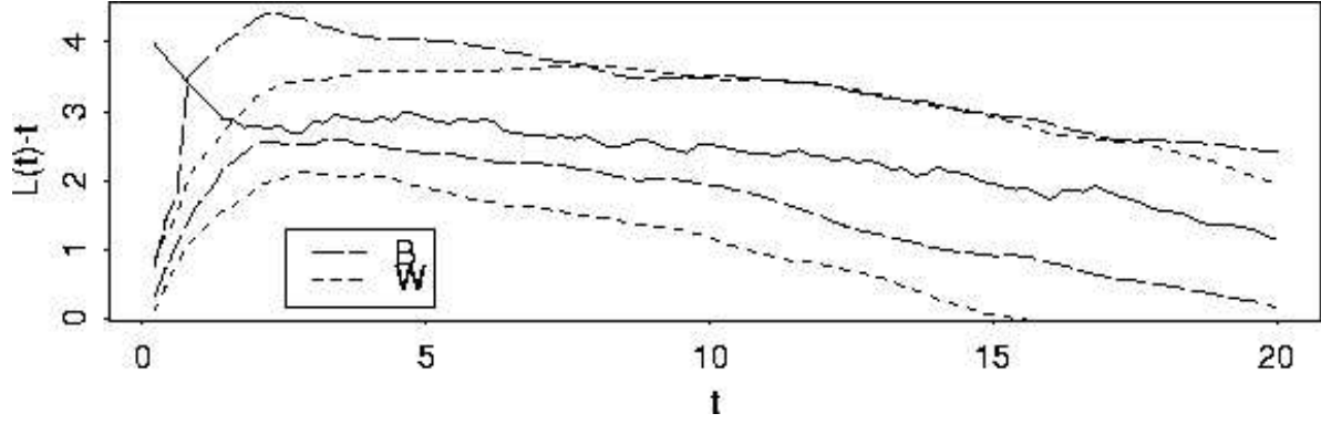
Fig. 5. Estimated L_{\text{inhom}}(t) - t (solid line) versus t (measured in km) under models B and model W.
