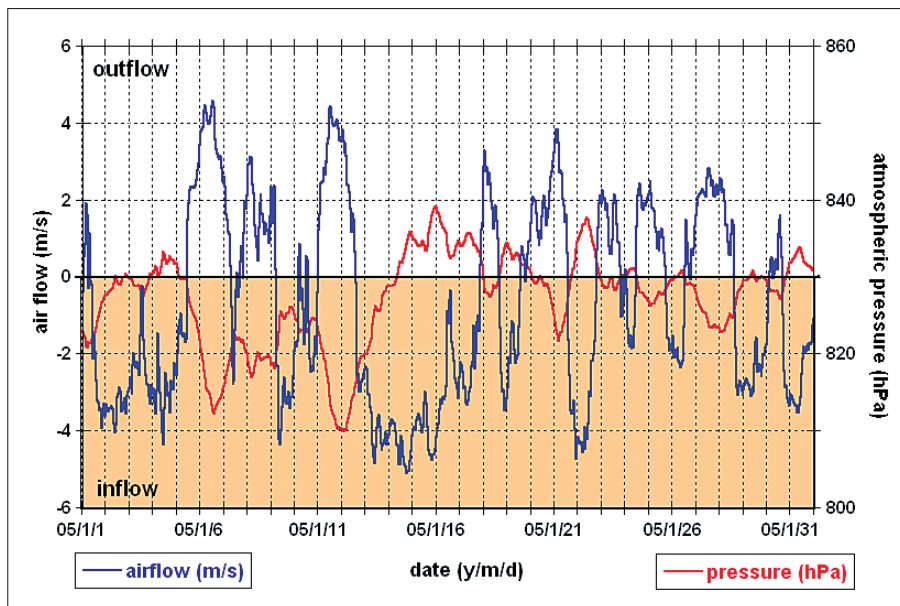
Fig. 5: Course of air flow direction and velocity at the Historic Entrance of Jewel Cave, as well as air pressure in the administration building at Jewel Cave NM. Measured from 1-31 January 2005 with an ultrasonic anemometer (10 Hz and averaging time of 10 s).
