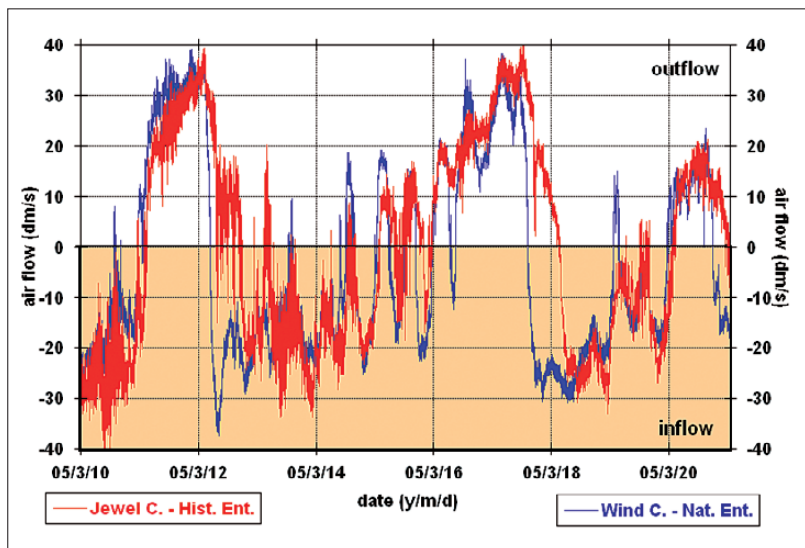
Fig. 14: Course of air flow direction and velocity at the Historic Entrance of Jewel Cave and at the Natural Entrance of Wind Cave from 10-21 March 2005, measured with an ultrasonic anemometer (10 Hz and averaging time of 10 s).
