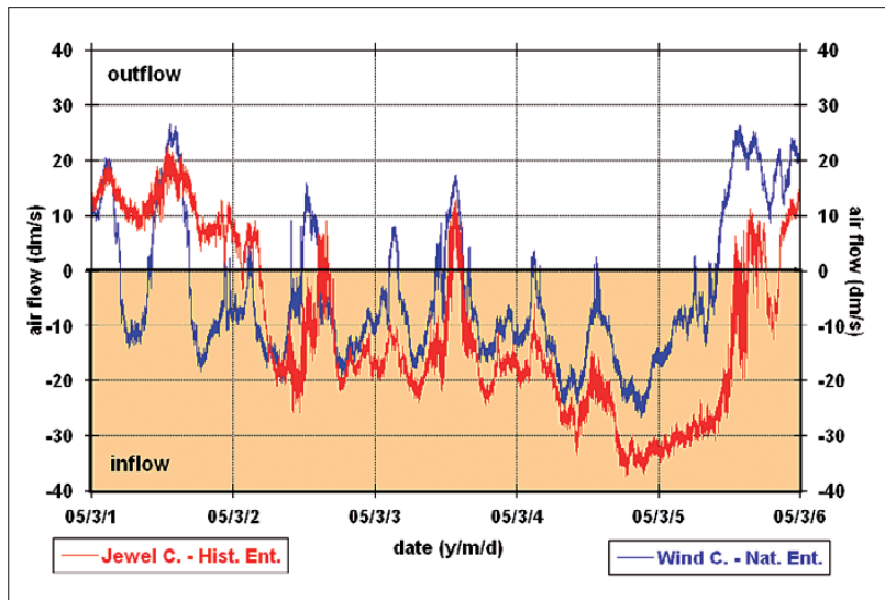
Fig. 13: Course of air flow direction and velocity at the Historic Entrance of Jewel Cave and at the Natural Entrance of Wind Cave from 1-6 March 2005, measured with an ultrasonic anemometer (10 Hz and averaging time of 10 s).
