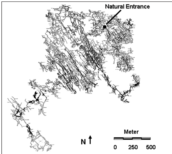
Fig. 6: Outline of Wind Cave, South Dakota (USA). Reference: Wind Cave National Park Service, with own additions.
