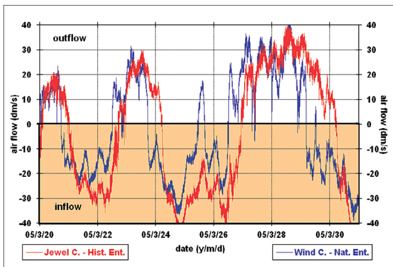
Fig. 15: Course of air flow direction and velocity at the Historic Entrance of Jewel Cave and at the Natural Entrance of Wind Cave from 20-31 March 2005, measured with an ultrasonic anemometer (10 Hz and averaging time of 10 s).
