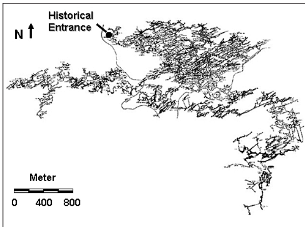
Fig. 8: Outline of Jewel Cave, South Dakota (USA). Reference: Jewel Cave National Monument, with own additions.
