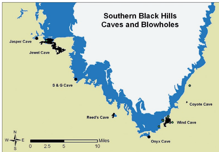
Fig. 1: Overview of the location of Jewel Cave and Wind Cave compared to different smaller caves (black dots and marks) and blow holes (green dots) showing the characteristic air flow pattern of barometric caves within the Southern Black Hills (South Dakota, USA). Brown: Madison Formation, blue: Minnelusa Formation.
