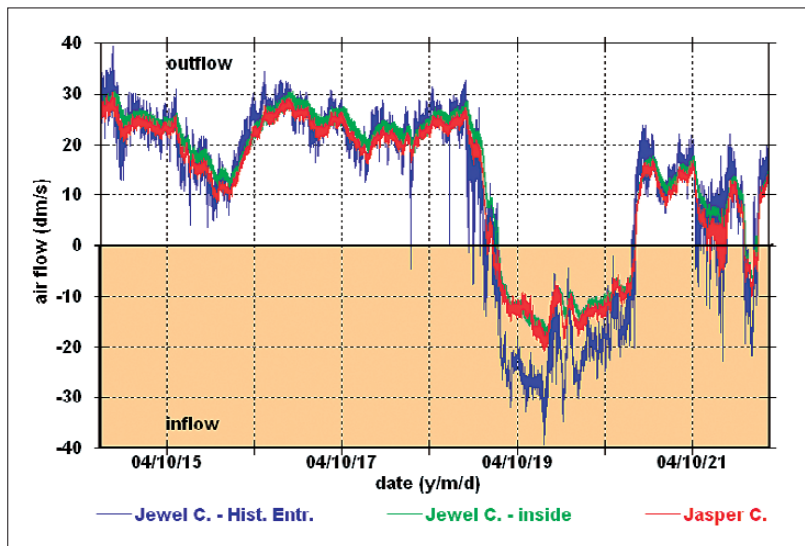
Fig. 18: Comparison of direction of air flow and velocity at the entrance areas of Jewel Cave and Jasper Cave. Measured from 14-22 October 2004 with an ultrasonic anemometer (10 Hz and averaging time of 15 s).
