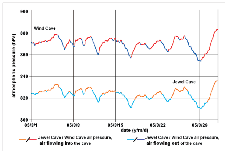
Fig. 12: Course of atmospheric pressure at Jewel Cave and Wind Cave in relationship to the air flow direction at the entrances of the two caves, March 2005.
