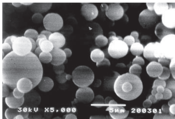
Figure 2. Typical distribution of \text{SiO}_2 particles obtained by the spray pyrolysis.
