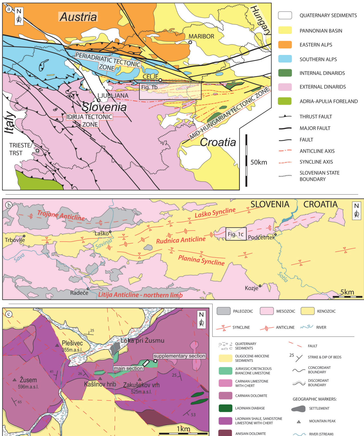
Fig. 1. a) Geotectonic subdivision of the Alpine-Dinaric-Pannonian transition zone with axes of the Sava Folds (compiled from Placer, 1999, 2016); boxed area is enlarged in Figure 1 b. b) Eastern Sava Folds with positions of major structures marked (simplified from Buser, 1978; Aničić and Juriša, 1985a); boxed area is enlarged in Figure 1 c (national border follows the Sotla River). c) Geological map of the eastern part of the Rudnica Anticline (after Aničić et al., 2004) with positions of studied sections marked.
