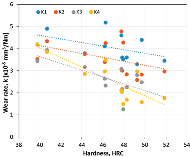
Figure 9: Dependence of the investigated hot-work tool steel's wear rate on the hardness under dry-sliding contact and different contact conditions
