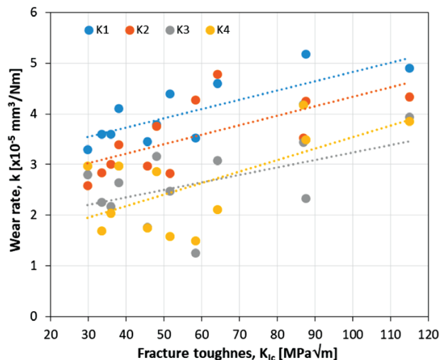
Figure 10: Dependence of the investigated hot-work tool steel's wear rate on the fracture toughness under dry-sliding contact and different contact conditions
