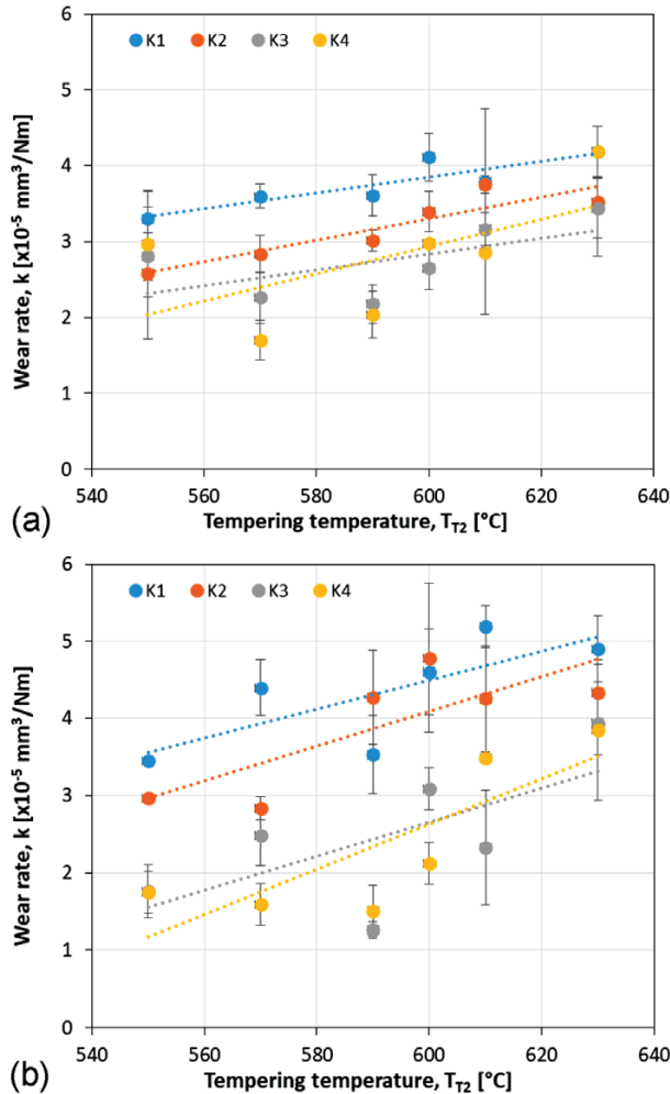
Figure 3: Influence of tempering temperature and contact conditions on wear rate for: a) austenitizing temperatures of 990 ^{\circ}\text{C} and b) 1030 ^{\circ}\text{C}
