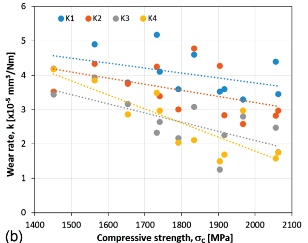
Figure 11: Dependence of the investigated hot-work tool steel's wear rate on bending and compressive strength under dry sliding contact and different contact conditions
