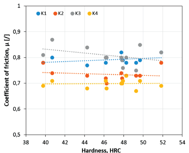
Figure 5: Dependence of the investigated hot-work tool steel coefficient of friction on hardness under dry-sliding contact and different contact conditions
