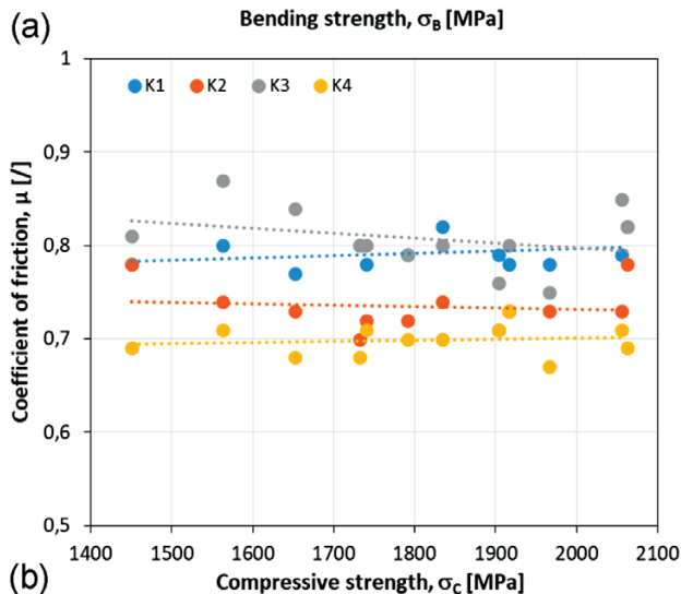
Figure 7: Dependence of the investigated hot-work tool steel coefficient of friction on bending and compressive strength under dry-sliding contact and different contact conditions
