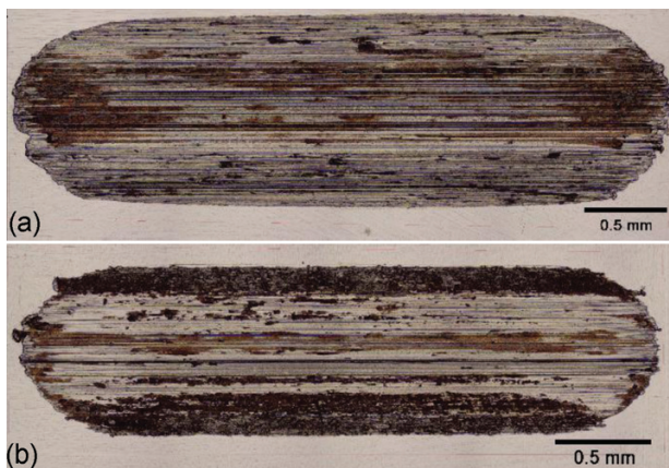
Figure 4: Typical wear scars; a) A6, p_H = 1100 \text{ MPa} , v_s = 0.01 \text{ m/s} ; b) A6, p_H = 800 \text{ MPa} , v_s = 0.12 \text{ m/s}
