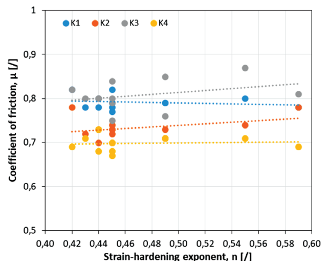
Figure 8: Dependence of the investigated hot-work tool steel's coefficient of friction on strain-hardening exponent under dry-sliding contact and different contact conditions
