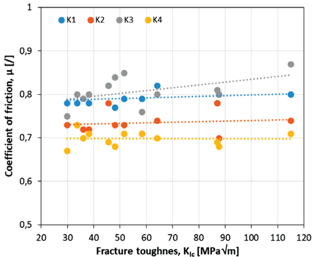
Figure 6: Dependence of the investigated hot-work tool steel coefficient of friction on fracture toughness under dry-sliding contact and different contact conditions
