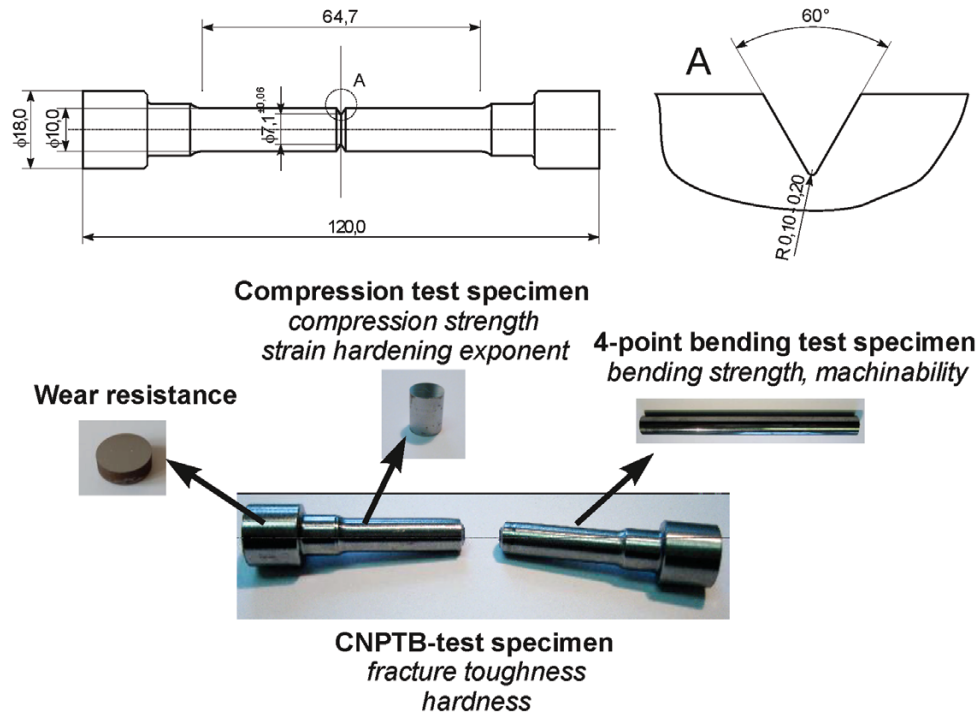
Figure 1: CNPTB master specimen and extracted specimens
