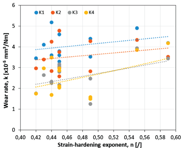
Figure 12: Dependence of the investigated hot-work tool steel's wear rate on strain-hardening exponent under dry-sliding contact and different contact conditions
