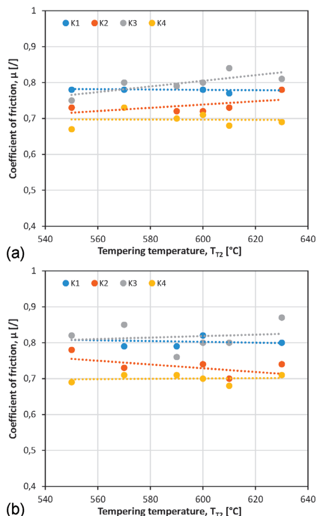
Figure 2: Influence of tempering temperature and contact conditions on steady-state coefficient of friction for: a) austenitizing temperatures of 990 °C and b) 1030 °C
